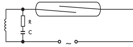
Fig. 17.1.2: AC voltage contact protection
